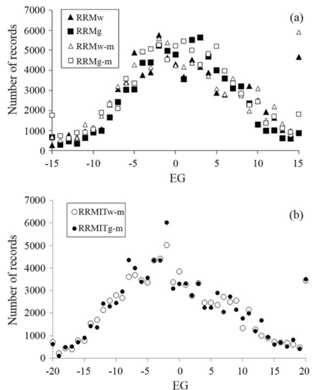
Figure 1 - Number of records analyzed in each environmental group for RRMw, RRMg, RRMw-m and RRMg-m (a) and RRMITw-m and RRMITg-m (b).
